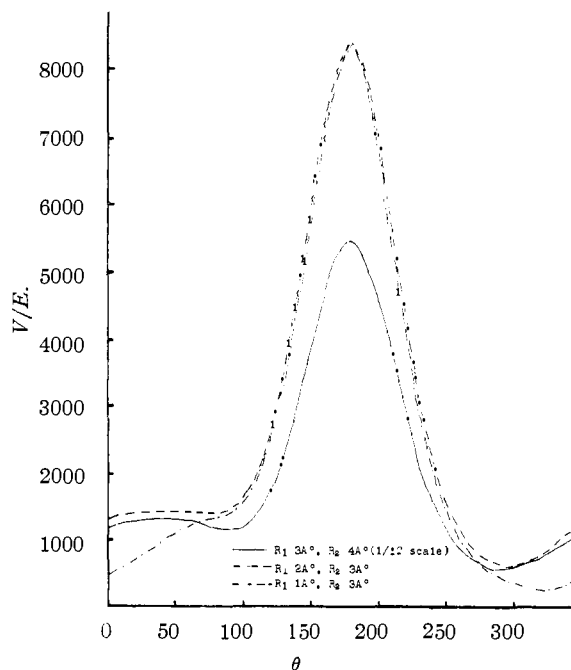
Fig. 2.—Potential energy vs. conformational angle \theta (as given by eq. 5).
